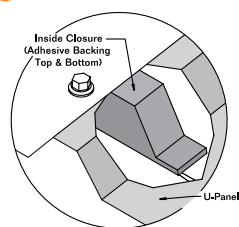
U Panel Closure Detail
