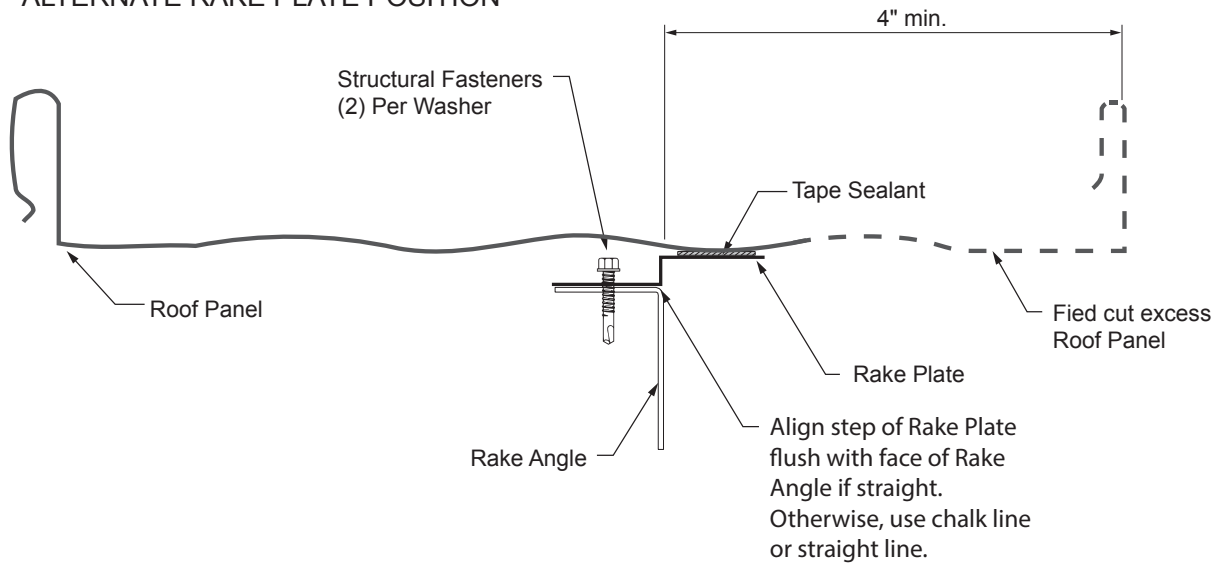
ALTERNATE RAKE PLATE POSITION
