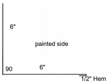
MTL Sidewall Flashing
