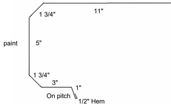
MTL Standard Gutter
