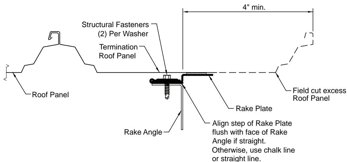
STANDARD RAKE PLATE POSITION
