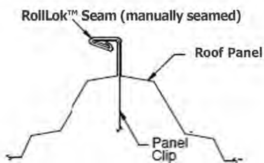
Panel Clips & Panel Ends
