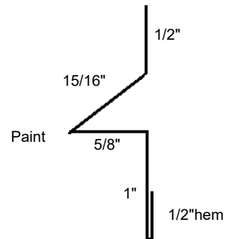
MTL Floating Rake Slide
