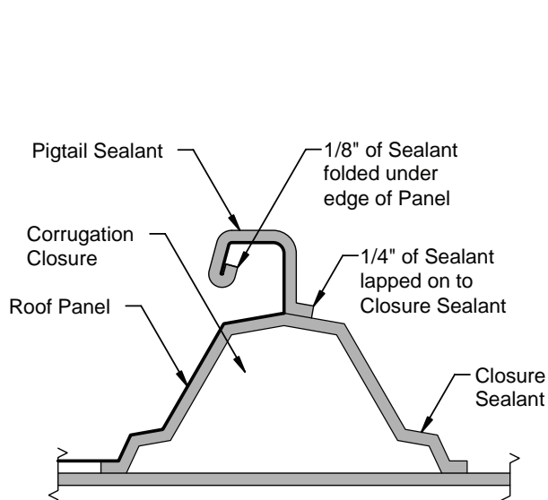
EAVE PIGTAIL SEALANT DETAIL
