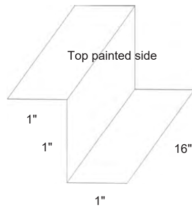
MTL Gutter Support Bracket
