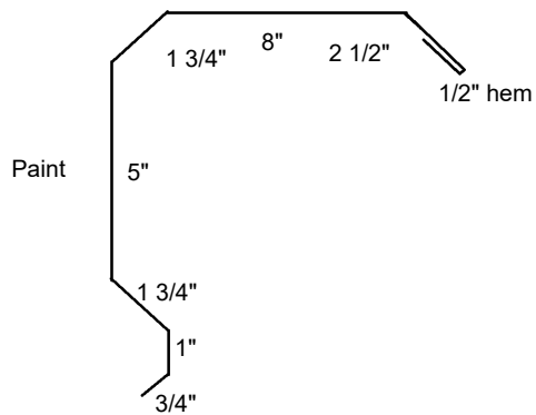
MTL Floating Rake
