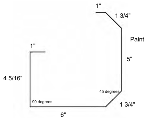
MTL Standard Gutter
