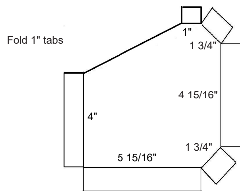
MTL Standard Gutter End- LH or RH
