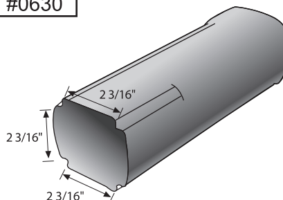
Sculptured Downspout
