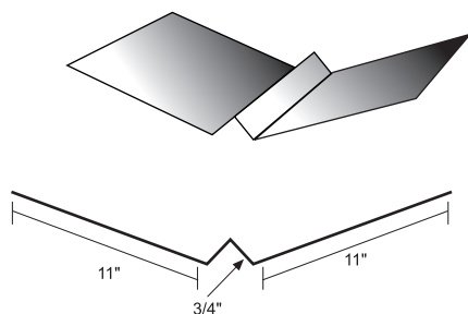
Sculptured Sleeve
