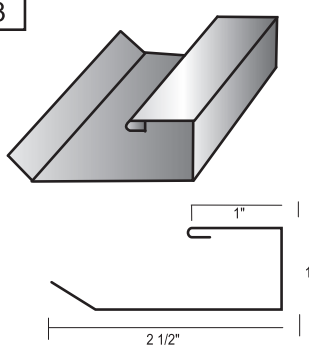
Adjustable Gable Strip Profile
