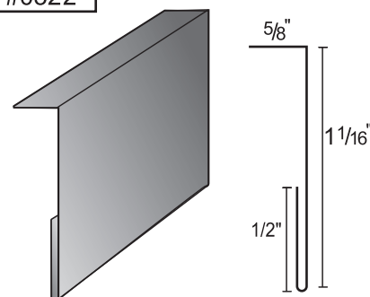
Sidewall Flashing
