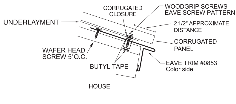
SECTION VIEW
