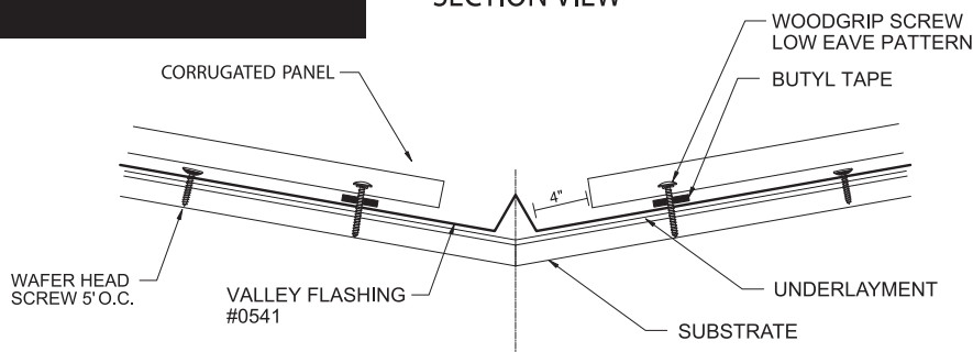
SECTION VIEW
