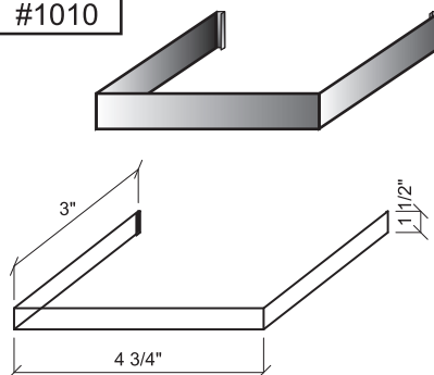
Gutter Strap
