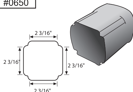
Sculptured Sleeve
