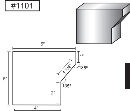
Eave Trim
