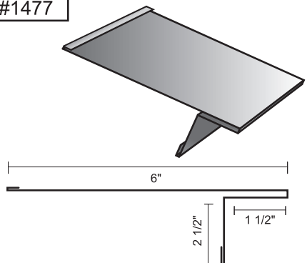
Adjustable Gable Trim Profile
