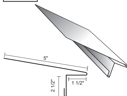
High Side Residential Eave Trim
