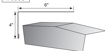
Peak Box for 1470, 1480
