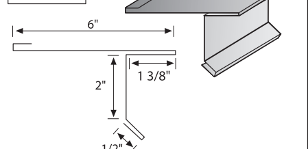
House Roof Rake
