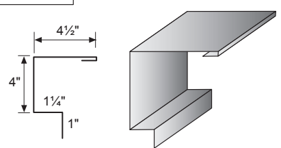
Drip Flashing
