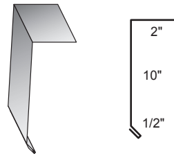
IS Partition Angle - 13" #1502
