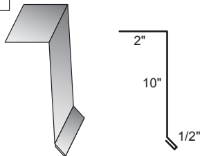
Partition Rake - 13" #1501
