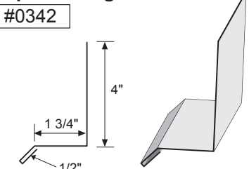
Drip Flashing
