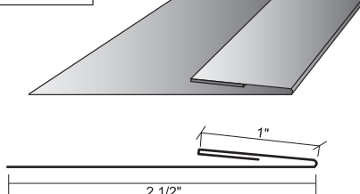
UPN House Roof Rake
