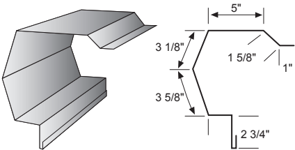
Lean to Rake Trim #1448
