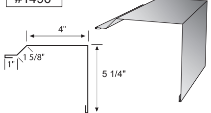
UPN Roof Rake - 10"
