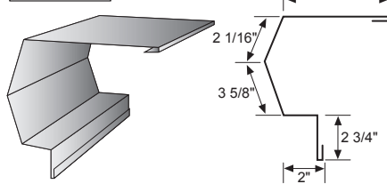
Lean to Rake Trim #1449
