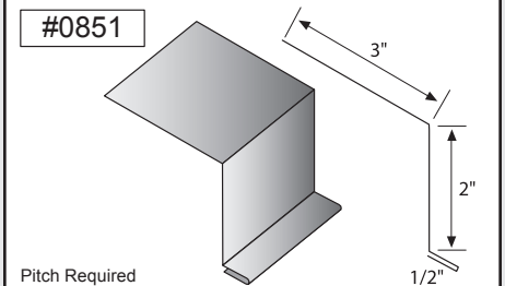
House Roof Eave Trim
