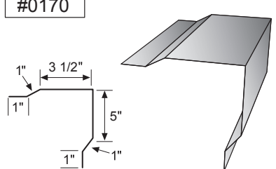
Outside Sculptured Corner
