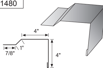
UPN House Roof Rake
