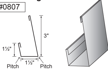
Soffit IS Angle
