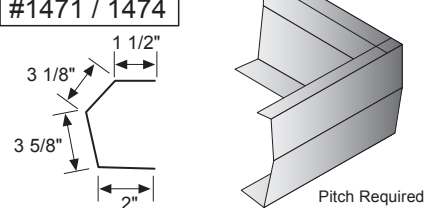
Corner Box for 1440 to 0500-0520 #1471 / 1474
