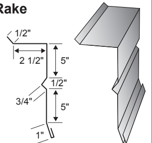
UPN Sculptured Rake - 17.75" #1498
