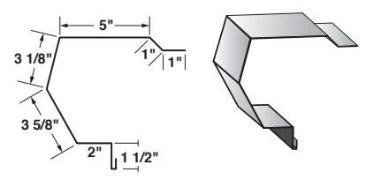
UPN Sculptured Rake - 17.75" #1498
