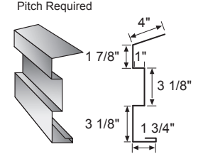
Greenhouse Skylight Screw Strap
