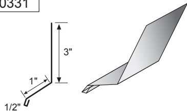
Drip Flashing – 5"
