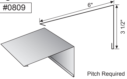
High Side Eave Trim
