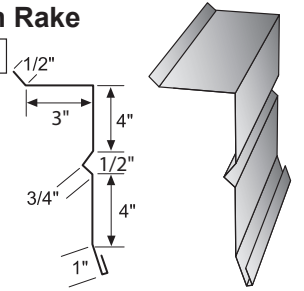
Partition Rake #1503
