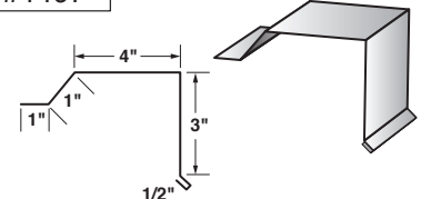
UPN Roof Rake - 10"
