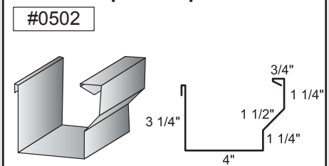
Residential Gutter – 13" uses stamped strap
