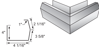
Outside Corner Box #1463 for 0503 & 0523
