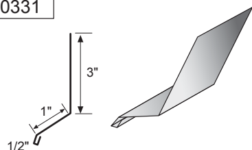
Drip Flashing – 5"
