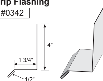
Drip Flashing
