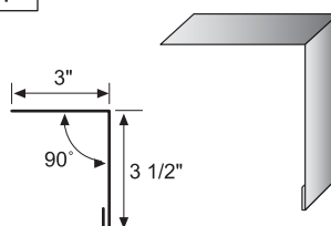
Eave – 7"
