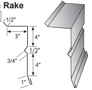
Partition Rake
