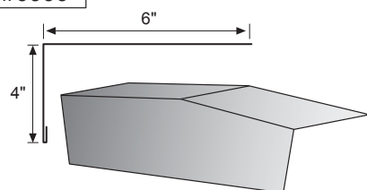
Peak Box for 1470, 1480
