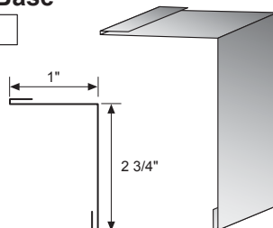
Fence Base
