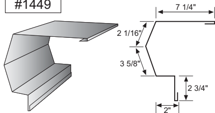
Lean to Rake Trim
