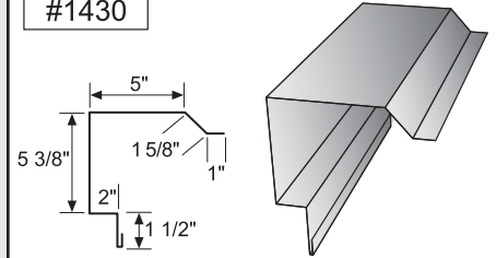
RPN Sculptured Rake
