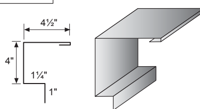
Drip Flashing
