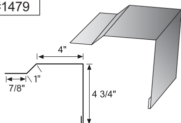
UPN Rake for #0800 Eave
