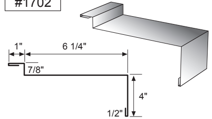
RUD Flashing 13.125"
