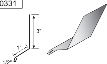
Drip Flashing – 5"
