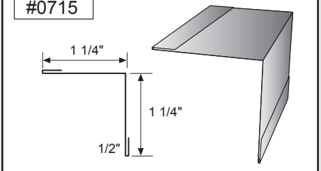
SS Rake Support Angle
