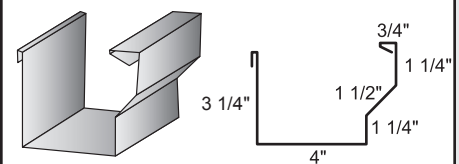
Residential Gutter – 13" uses stamped strap
