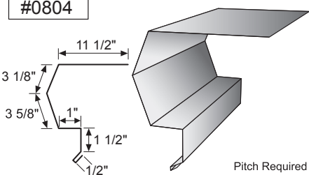
MTL Gutter Bracket - 3"
