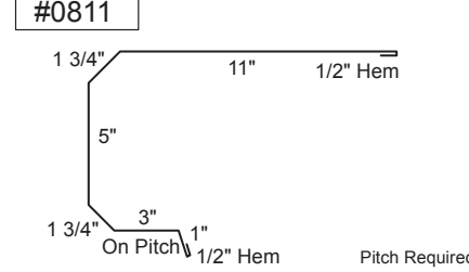
MTL Gutter Endcap
