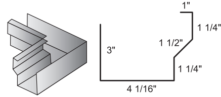
Inside Corner Box for 0503 & 0523
