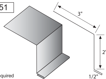
House Roof Eave Trim
