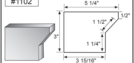
Gutter Endcap for 0502
