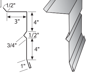
Partition Rake
