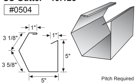
SS Gutter - 19.125"
