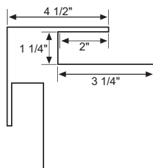
Boxed Corner 22"
