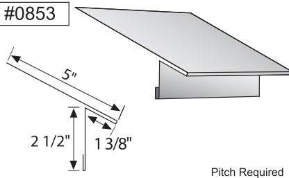
House Roof Eave Trim
