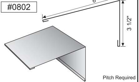
High Side Eave Trim
