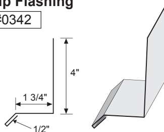
Drip Flashing
