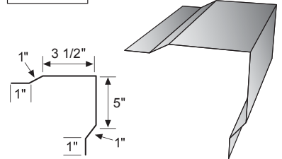
RUD Flashing 13.125"
