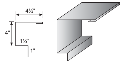
Eyebrow Soffit Cover 12.25"
