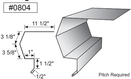
SS High Side Eave
