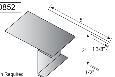
House Roof Eave Trim
