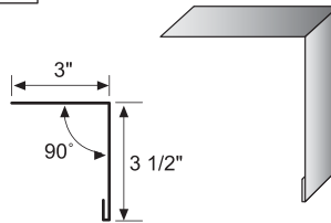
IS Rake – 12"
