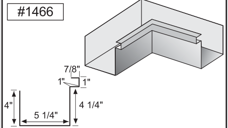
Inside Corner Box for 0510
