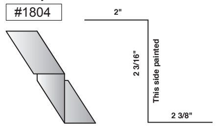
SS Hip Closure
