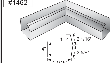
Inside Corner Box for 0503 & 0523
