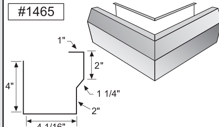
Outside Corner Box for 0501
