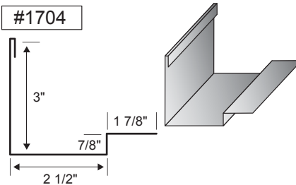
Soffit Cover
