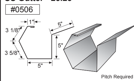
SS Gutter - 23.25"
