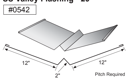
SS Valley Flashing - 29"
