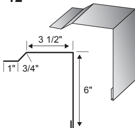
OS Rake – 12"
