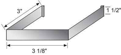
Downspout Strap
