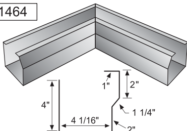
Inside Corner Box for 0501
