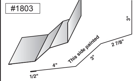
SS Endwall
