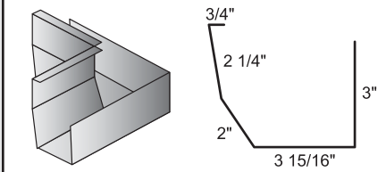
Outside Corner Box for 0503 & 0523
