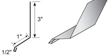
OS Rake – 12"
