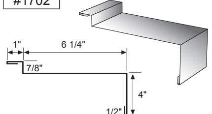
RUD Flashing 13.125"
