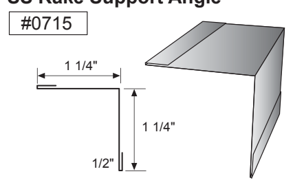
SS Rake Support Angle
