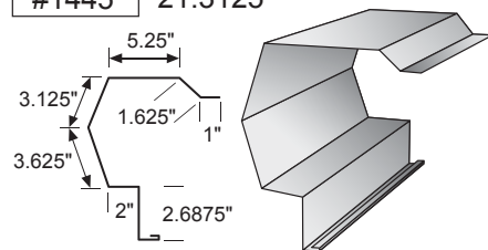
IS Corner Box for #0500 & 0520
