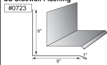
SS Sidewall Flashing
