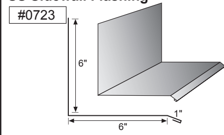
SS Sidewall Flashing
