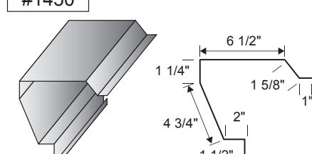
Sculptured Rake Trim
