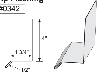
Drip Flashing
