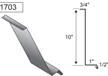
IS Rake
