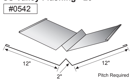
SS Valley Flashing - 29"
