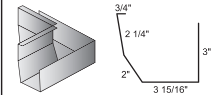
Outside Corner Box for 0503 & 0523
