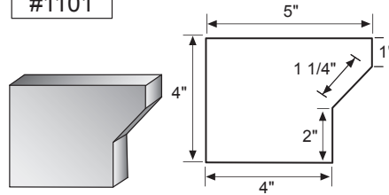
Gutter Endcap for 0501
