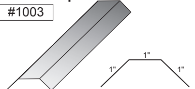
Greenhouse Skylight Screw Strap
