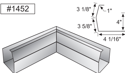
IS Corner Box for #0500 & 0520
