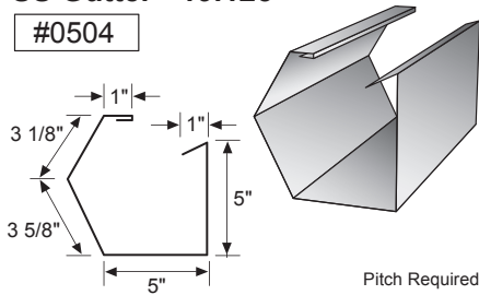
SS Gutter - 19.125"
