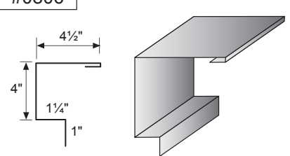
Eyebrow Soffit Cover 12.25"
