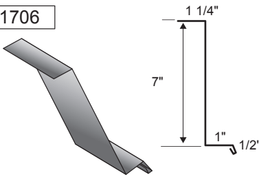
IS Rake
