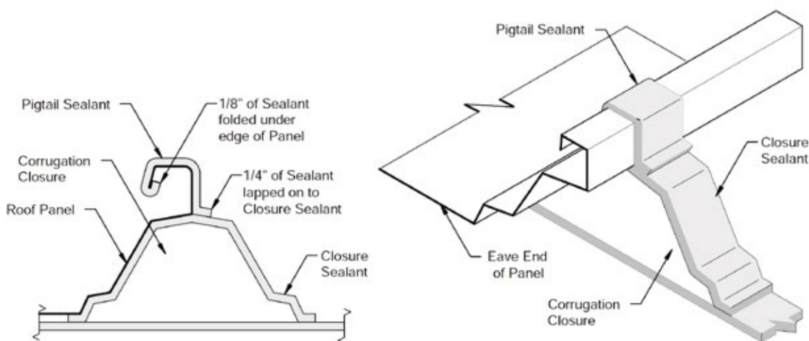
EAVE PIGTAIL SEALANT DETAIL
