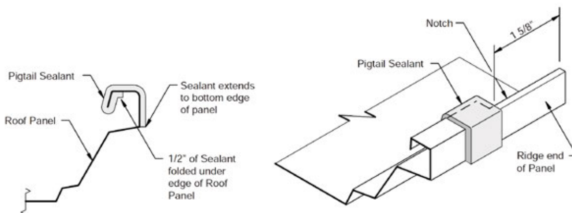
RIDGE PIGTAIL SEALANT DETAIL
