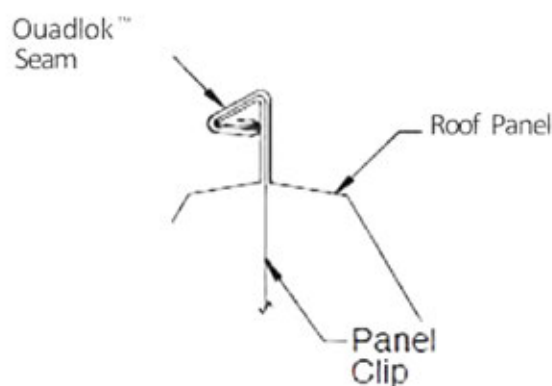
@ Panel Clips
