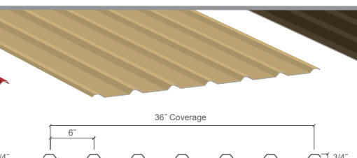
U Panel
