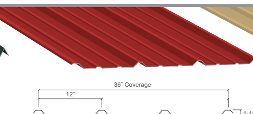
R Panel
