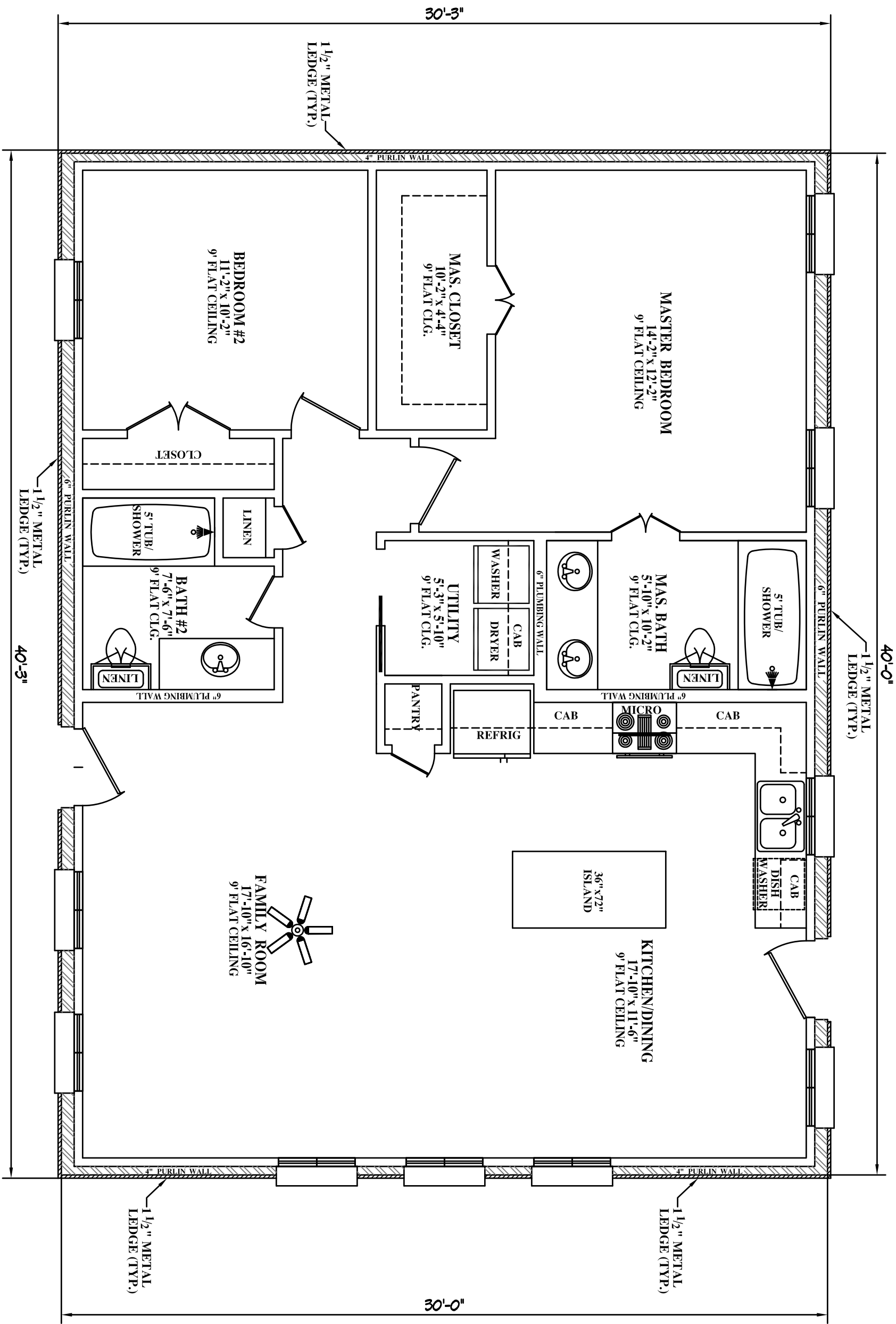
FLOOR PLAN 1/4"=1'-0"
