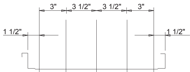
Screw Spacing at Eave
