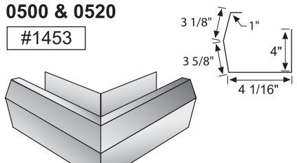
Outside Corner Box for 0500 & 0520
