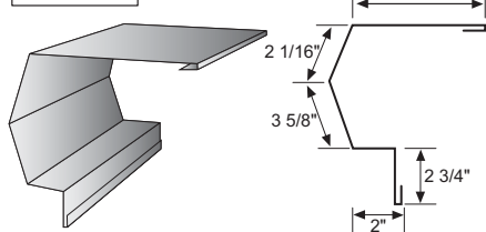
Lean to Rake Trim
