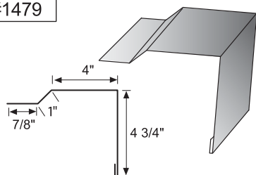
UPN Rake for #0800 Eave
