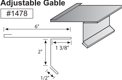
House Roof Rake
