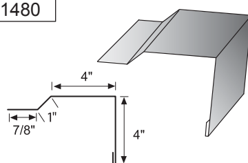
UPN House Roof Rake
