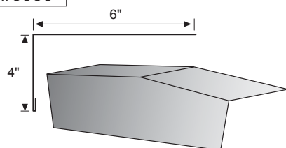
Peak Box for 1470, 1480 and 1490 Rake
