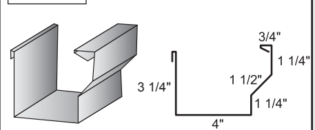
Residential Gutter – 13" uses stamped strap
