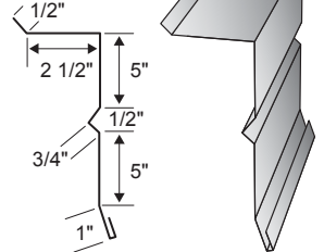
UPN Sculptured Rake - 17.75"
