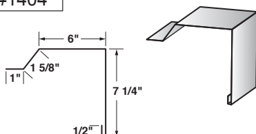
Loafing Shed Rake - 16.375"
