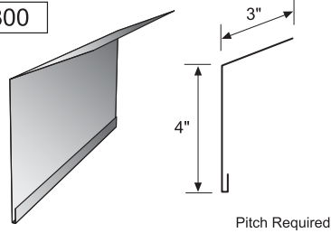
Utility Eave Trim
