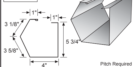
Utility Gutter Profile
