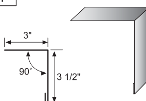
Eave – 7"
