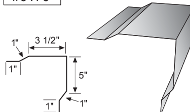
Outside Sculptured Corner
