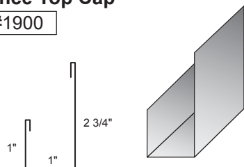
Fence Top Cap
