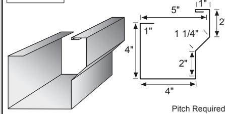
Residential Gutter Profile
