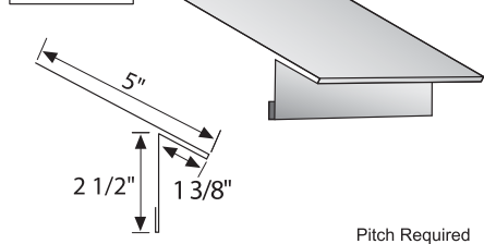
House Roof Eave Trim
