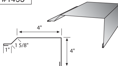
House Roof Rake w/Hem
