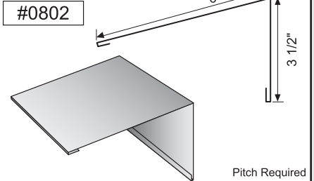
High Side Eave Trim
