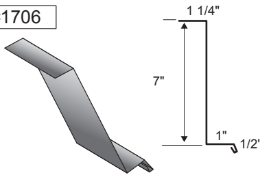
IS Rake
