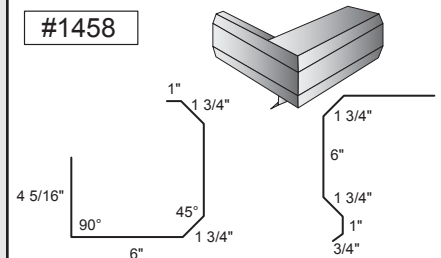
MTL Corner Box
