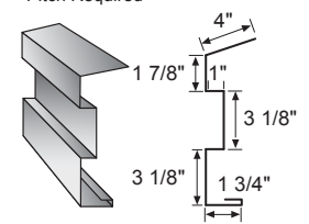
Greenhouse Skylight Screw Strap
