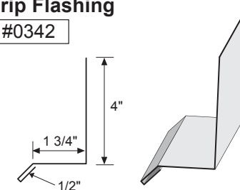
Drip Flashing
