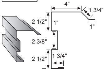
Loafing Shed Rake - 16.375"
